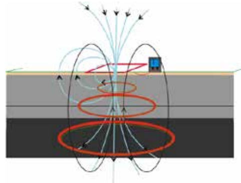
The principle of a TEM survey: A current cut-off in the transmitter loop emits an electromagnetic transient that induces secondary fields (eddy currents) in conductive structures. The receiver coil intercepts the transient and the resulting voltage decay is digitally recorded.
